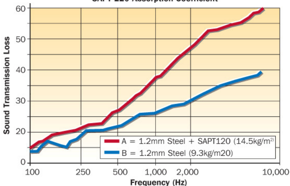
SAPT 220 Absorption Coefficient
